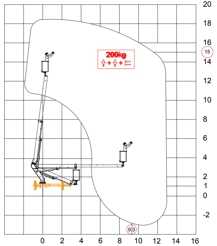
MERAJ Working Diagram Max. values and repeatability can change within ±5% due to manufacturing variance. This drawing is the property of Meraj® and should not be used or shared other than the person intended nor replicated without permission. MTBP-15
